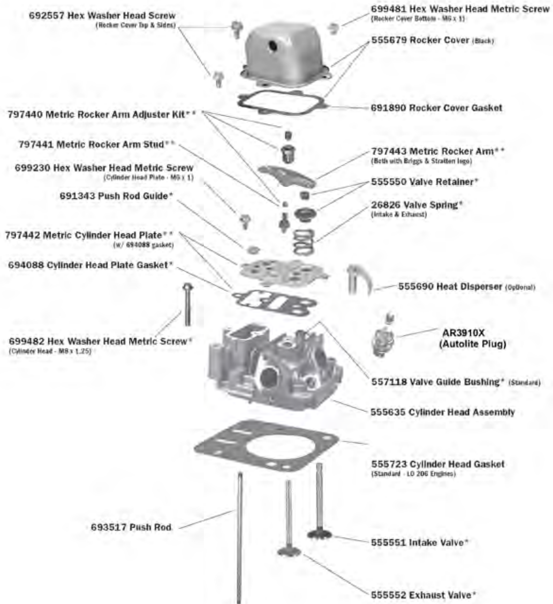
555635 Cylinder Head Assembly
