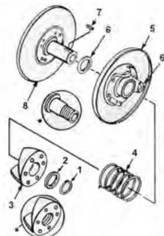
40/44D Driven Unit
